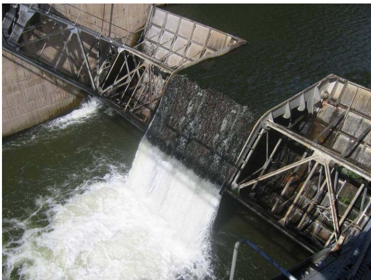
Vanne segment (L = 22 m, H = 6 m) Poussée = 500 t
